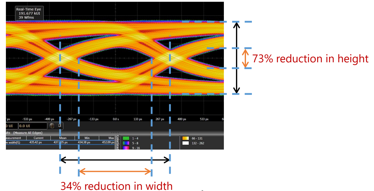
Eye Diagram at Output of Cable
